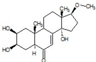
Methyl-dihydro-rubrosterone
