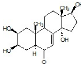
Dihydro-rubrosterone
